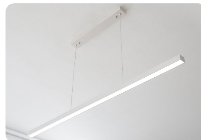
DY79-03 Name SL15W-6500K Watt LED 60W Kelvin 6500K Size 1502 × 40 × 30
