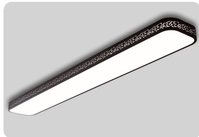
DY112-02 Name Kitchen lights Watt LED 60W Kelvin 6500K / 4000K Size 1185 × 165 × 70
