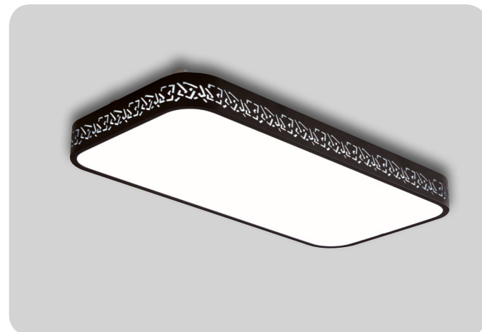
DY112-01 Name Room lights Watt LED 30W Kelvin 6500K / 4000K Size 500 × 250 × 70
