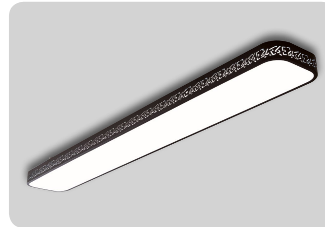
DY113-01 Name Kitchen lights Watt LED 30W Kelvin 6500K / 4000K Size 950 × 165 × 70
