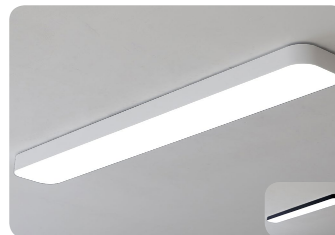
DY67-01 Name Kitchen lights Watt LED 60W Kelvin 6500K / 4000K Size 1188×165×47
