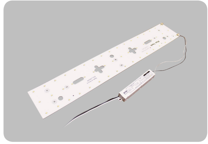
DY89-04 Name LED Reform Module Watt LED 25W Kelvin 6500K / 4000K / 3000K Size 580x100
