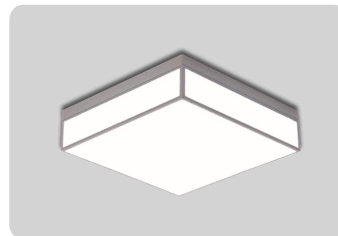
DY87-07 Name Artsol (Big size) Watt LED 25W Kelvin 6500K / 4000K Size 320×320×85
