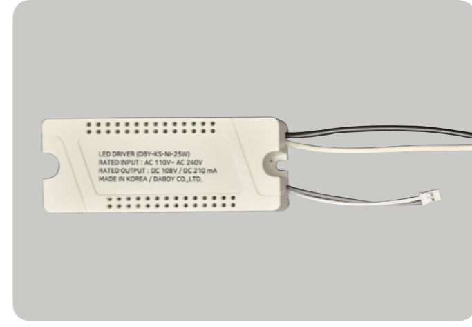
DY100-06-25W Name NON INSULATION CONVERTER (DRIVER) Watt LED 25W
