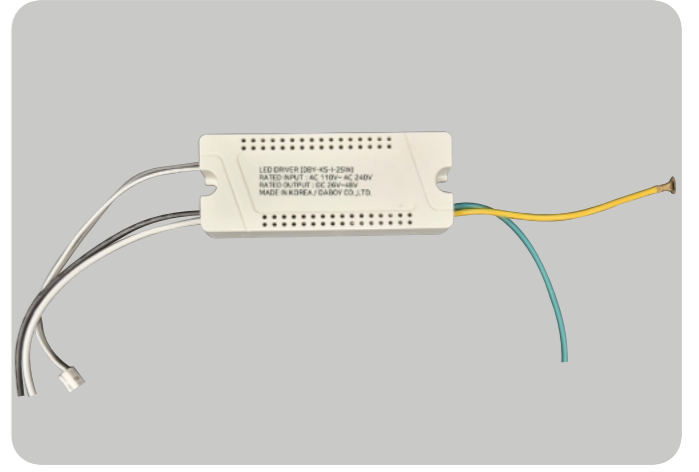
DY100-05-25W Name INSULATION CONVERTER (DRIVER) Watt LED 25W
